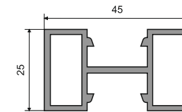
AMPP-26 Divider Profile (Male - Female) Size: 3 Mtr. Finish: Black Matt / Brushed Gold
