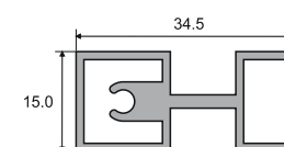
AMAP-31 Top Shutter Profile Size: 3 Mtr. | Glass Size: 4 to 6 mm Finish: Black Matt / Brushed Gold
