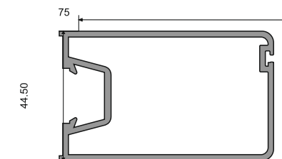
AMPP-31 Still Door Fix Profile Size: 3 Mtr. Finish: Black Matt / Brushed Gold
