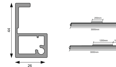
AMAP-35 - Frame Profile Handle AMAP-36 - 200 mm Handle AMAP-37 - 1200mm Handle Left & Right Size: 3 Mtr. | Glass Size: 4 mm Finish: Black Matt / Brushed Gold
