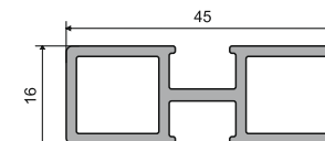
AMPP-03 Divider Profile Size: 3 Mtr. Finish: Black Matt / Brushed Gold
