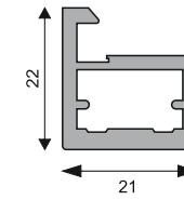
AMAP-19 Profile Size: 3 Mtr. | Glass Size: 4 mm Finish: Black Matt / Brushed Gold
