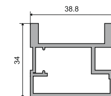
AMAP-10 Shutter Handle Profile Size: 2.5 - 3 Mtr. | Glass Size: 4 to 6 mm Finish: Black Matt / Brushed Gold
