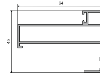
AMPP-09 Door Inner Frame Size: 3 Mtr.
