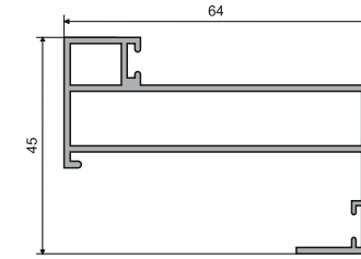
AMPP-10 Door Inner Frame Size: 3 Mtr.
