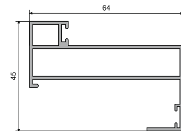
AMPP-10 Door Inner Frame Size: 3 Mtr. Finish: Black Matt / Brushed Gold
