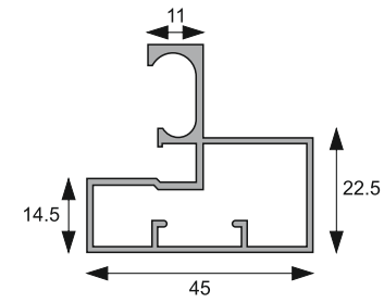
AMAP-28 Frame- Handle Profile Size: 3 Mtr. | Glass Size: 4 mm Finish: Black Matt / Brushed Gold
