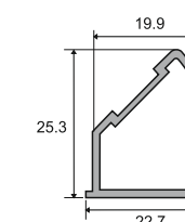
AMAP-38 Corner Profile Size: 3 Mtr. | Glass Size: 4 to 6 mm Finish: Black Matt / Brushed Gold
