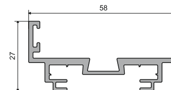
AMPP-07 Door Frame Profile Size: 3 Mtr. Finish: Black Matt / Brushed Gold
