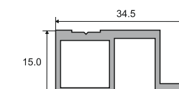
AMAP-33 Shutter Handle Profile Size: 3 Mtr. | Glass Size: 4 to 6 mm Finish: Black Matt / Brushed Gold
