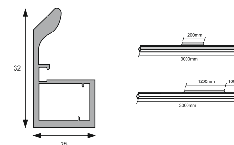
AMAP-05 - Handle Profile AMAP-06 - 200 mm Handle AMAP-22 - 1200mm Handle Left & Right
