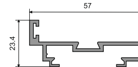
AMPP-07 Door Frame Profile Size: 3 Mtr. Finish: Black Matt / Brushed Gold
