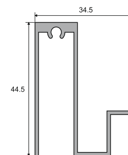
AMAP-30 Bottom Shutter Profile Size: 3 Mtr. | Glass Size: 4 to 6 mm Finish: Black Matt / Brushed Gold
