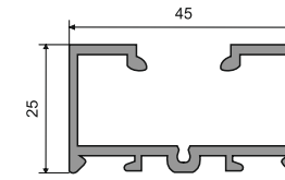
AMPP-21 Single Glaze Profile Size: 3 Mtr. Finish: Black Matt / Brushed Gold
