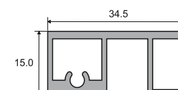
AMAP-31 Top Shutter Profile Size: 3 Mtr. | Glass Size: 4 to 6 mm Finish: Black Matt / Brushed Gold
