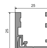
AMPP-33-34 Single Glaze Profile (Male - Female) Size: 3 Mtr. Finish: Black Matt / Brushed Gold
