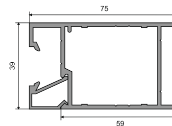
AMPP-29-30 Still Door Profile (Male - Female) Size: 3 Mtr. Finish: Black Matt / Brushed Gold
