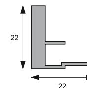
AMAP-02 Top-Bottom Profile Size: 250, 348, 398, 448, 498, 548, 598, 748, 898 mm Finish: Black Matt / Brushed Gold / Grey Matt
