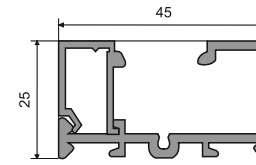
AMPP-22-23 Single Glaze Profile (Male - Female) Size: 3 Mtr. Finish: Black Matt / Brushed Gold
