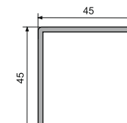
AMPP-08 Pole Profile Size: 3 Mtr. Finish: Black Matt / Brushed Gold
