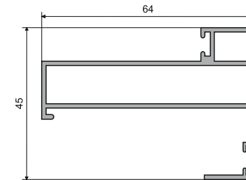
AMPP-09 Door Outer Frame Size: 3 Mtr. Finish: Black Matt / Brushed Gold
