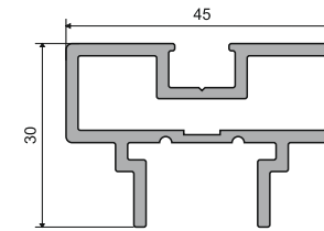
AMPP-02 Top-Bottom Size: 3 Mtr. | Glass Size: 8 mm Finish: Black Matt / Brushed Gold
