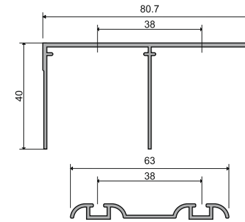
AMAP-14 Top Bottom Sliding Track Size: 2.5 Mtr. , 3.6 Mtr. Finish: Black Matt / Brushed Gold
