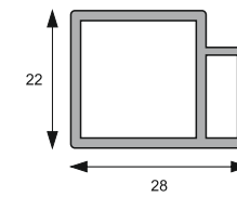
AMAP-23 Shelving Profile Size: 3 Mtr. | Glass Size: 5 mm Finish: Black Matt / Brushed Gold
