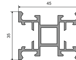
AMPP-18 Four Way Portal Profile Size: 3 Mtr. Finish: Black Matt / Brushed Gold
