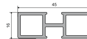
AMPP-03 Divider Profile Size: 3 Mtr. | Glass Size: 4 to 6 mm Finish: Black Matt / Brushed Gold
