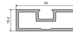
AMPP-01 Partition Profile Size: 3 Mtr. | Glass Size: 8 mm Finish: Black Matt / Brushed Gold
