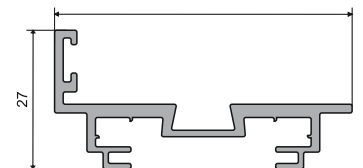
AMPP-07 Door Frame Profile Size: 3 Mtr.
