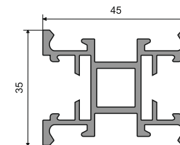
AMPP-18 Four Way Portal Profile Size: 3 Mtr. Finish: Black Matt / Brushed Gold
