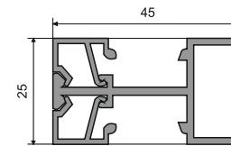
AMPP-27-28 Single Glaze Middle (Male - Female) Size: 3 Mtr. Finish: Black Matt / Brushed Gold
