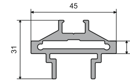
AMPP-39 Top-Bottom Size: 3 Mtr.
