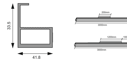
AMAP-40 - Profile Handle AMAP-41 - 200 mm Handle AMAP-42 - 1200mm Handle Left & Right Size: 3 Mtr. | Glass Size: 4 mm Finish: Black Matt / Brushed Gold
