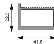
AMAP-39 Frame Profile Size: 3 Mtr. | Glass Size: 4 mm Finish: Black Matt / Brushed Gold
