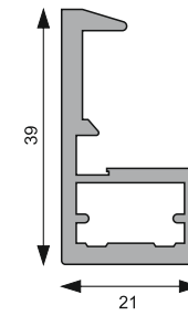
AMAP-20 - Profile Handle AMAP-21 - 200 mm Handle AMAP-29 - 1200mm Handle Left & Right Size: 3 Mtr. | Glass Size: 4 mm Finish: Black Matt / Brushed Gold
