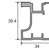
AMAP-17 Shutter Handle Profile Size: 2.5 Mtr. , 3 Mtr. | Glass Size: 4 to 6 mm Finish: Black Matt / Brushed Gold
