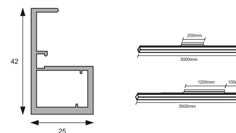
AMAP-27 Top-Bottom Profile Size: 3 Mtr. Finish: Black Matt / Brushed Gold
