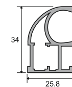
AMAP-15 Shutter Handle Profile Size: 2.5 Mtr. , 3 Mtr. | Glass Size: 4 to 6 mm Finish: Black Matt / Brushed Gold
