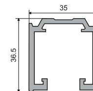
AMPP-05 Track Size: 8 Feet, 12 Feet Finish: Black Matt / Brushed Gold
