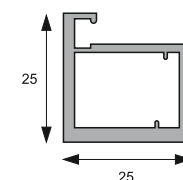
AMAP-04 Frame Profile Size: 3 Mtr. | Glass Size: 5 mm Finish: Black Matt / Brushed Gold
