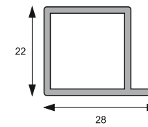
AMAP-09 Shelving Profile Size: 3 Mtr. | Wooden Shelf Size: 18 mm Finish: Black Matt / Brushed Gold
